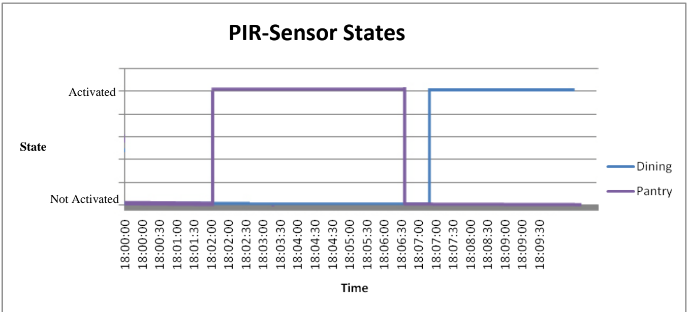
Figure B.6. Sensor States - PIR
