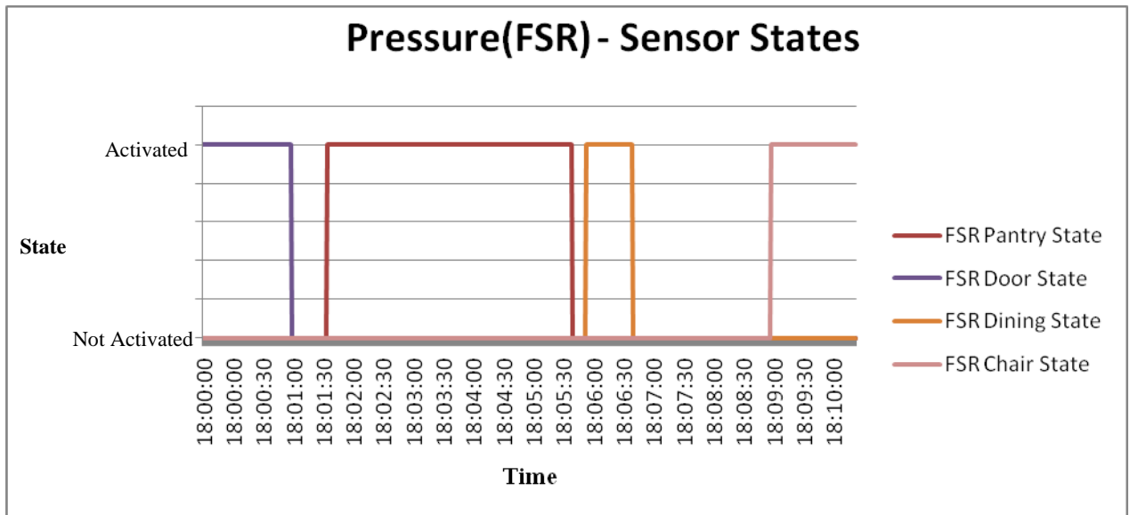
Figure B.2. Sensor States – Pressure(FSR)
